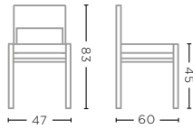
CHAIR FIONA G510-PE-AW (P. 67) TEAK NATURAL GREY / PE WICKER ANTIQUE WEED W47 X D60 X H83 CM
