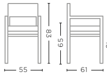
ARMCHAIR FIONA G510A-PE-AW (P. 42-43, 52-53, 66) TEAK NATURAL GREY / PE WICKER ANTIQUE WEED W55 X D61 X H83 CM
